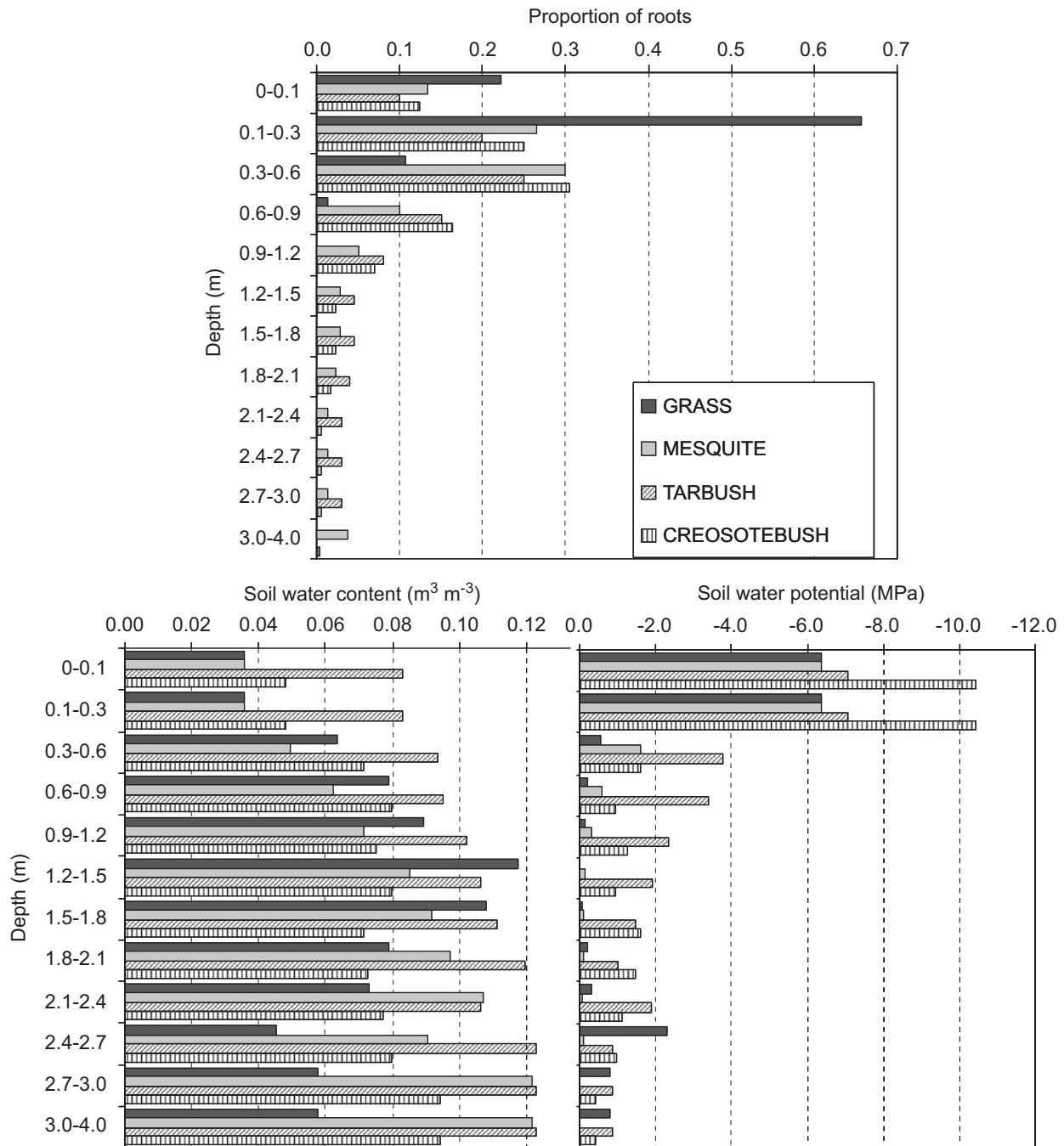
Fig. 2. Root profile for the vegetation types considered in this study (top). Initial soil water content ( m^3 m^{-3} ) (left bottom) and soil water potential (MPa) (right bottom).
