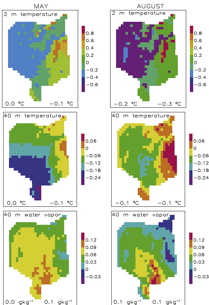
Fig. 5. Differences between 1858 and 1998 at 13:00 LST for 2 m temperature (°C) (top); first model level temperature (°C) (middle); water vapor mixing ratio ( \text{g kg}^{-1} ) (bottom). The area-averaged differences at 12:00 MST (left) and the diurnal average (right) are shown in each figure.
