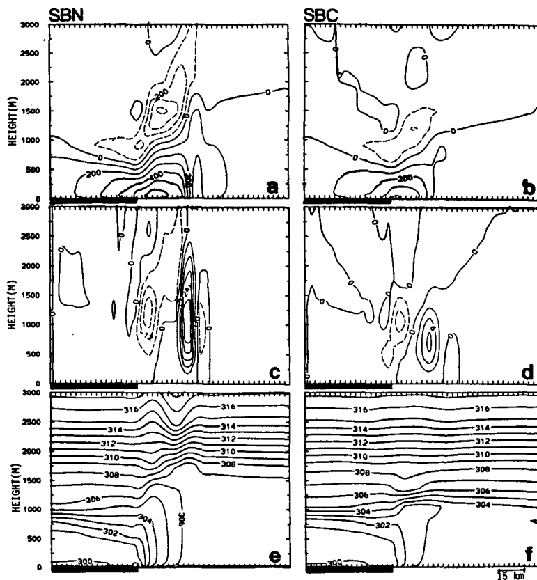
FIG. 4. Vertical cross section of the simulated domain for the cases SBN and SBC at 1400 LST for (a) and (b) u (west-east) component of the wind in \text{cm s}^{-1} ; (Dashed contours indicate negative component-easterly.) (c) and (d) the vertical wind component in \text{cm s}^{-1} ; (Dashed contours indicate negative component-downward vertical velocity.) (e) and (f) the potential temperature in ^{\circ}\text{K} . The dark segment indicates the sea section of the domain.
