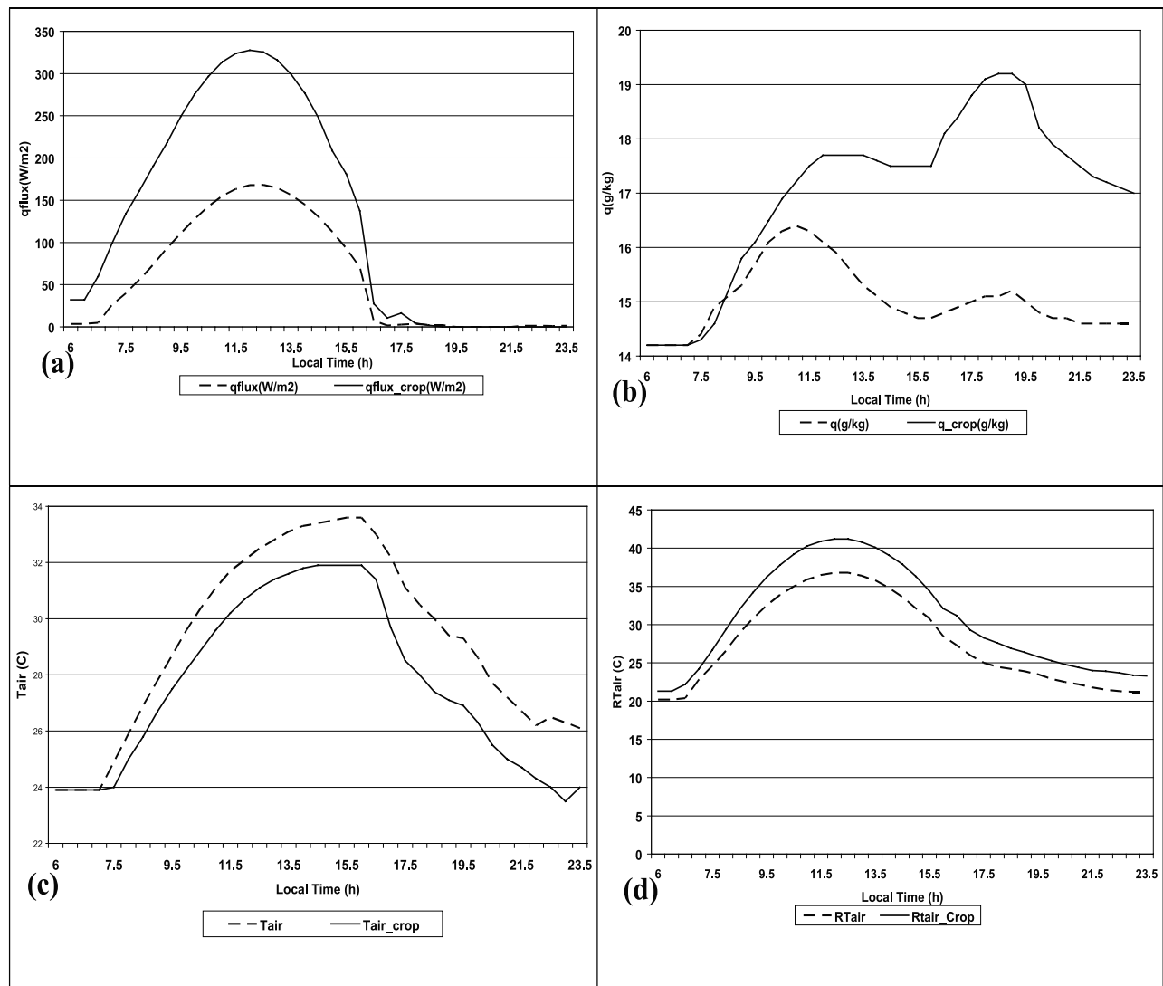
Figure 7. Results of model runs by the Land Surface-Boundary Layer Model for 15 March 1999 in Meerut, (a) latent heat flux (W/m 2 ), (b) specific humidity (g/kg), (c) air temperature (°C), and (d) radiometric temperature (°C). The suffix “crop” indicates model results for irrigated crop.
