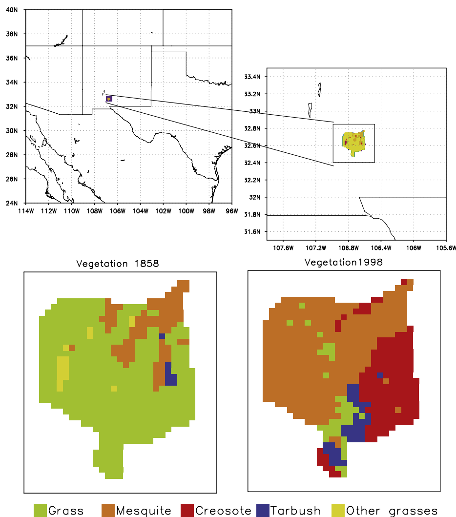
Fig. 1. Location of the Jornada Long-Term Experimental Range site, the GEMRAMS model domain for the simulations (top), and the vegetation distribution in 1858 and 1998 (bottom). Each grid cell is 1 \text{ km} \times 1 \text{ km} .
