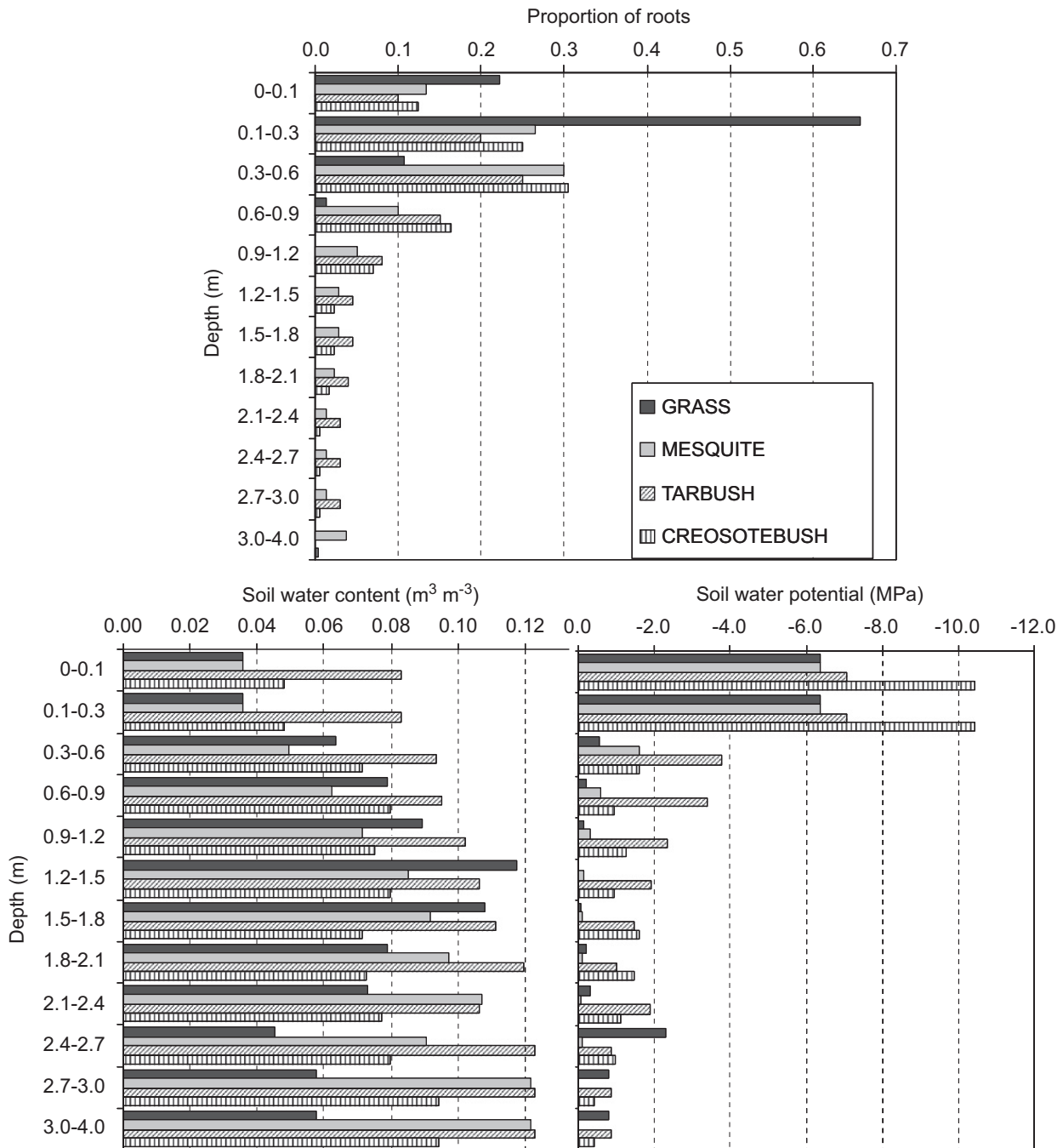
Fig. 2. Root profile for the vegetation types considered in this study (top). Initial soil water content ( m^3 m^{-3} ) (left bottom) and soil water potential (MPa) (right bottom).
